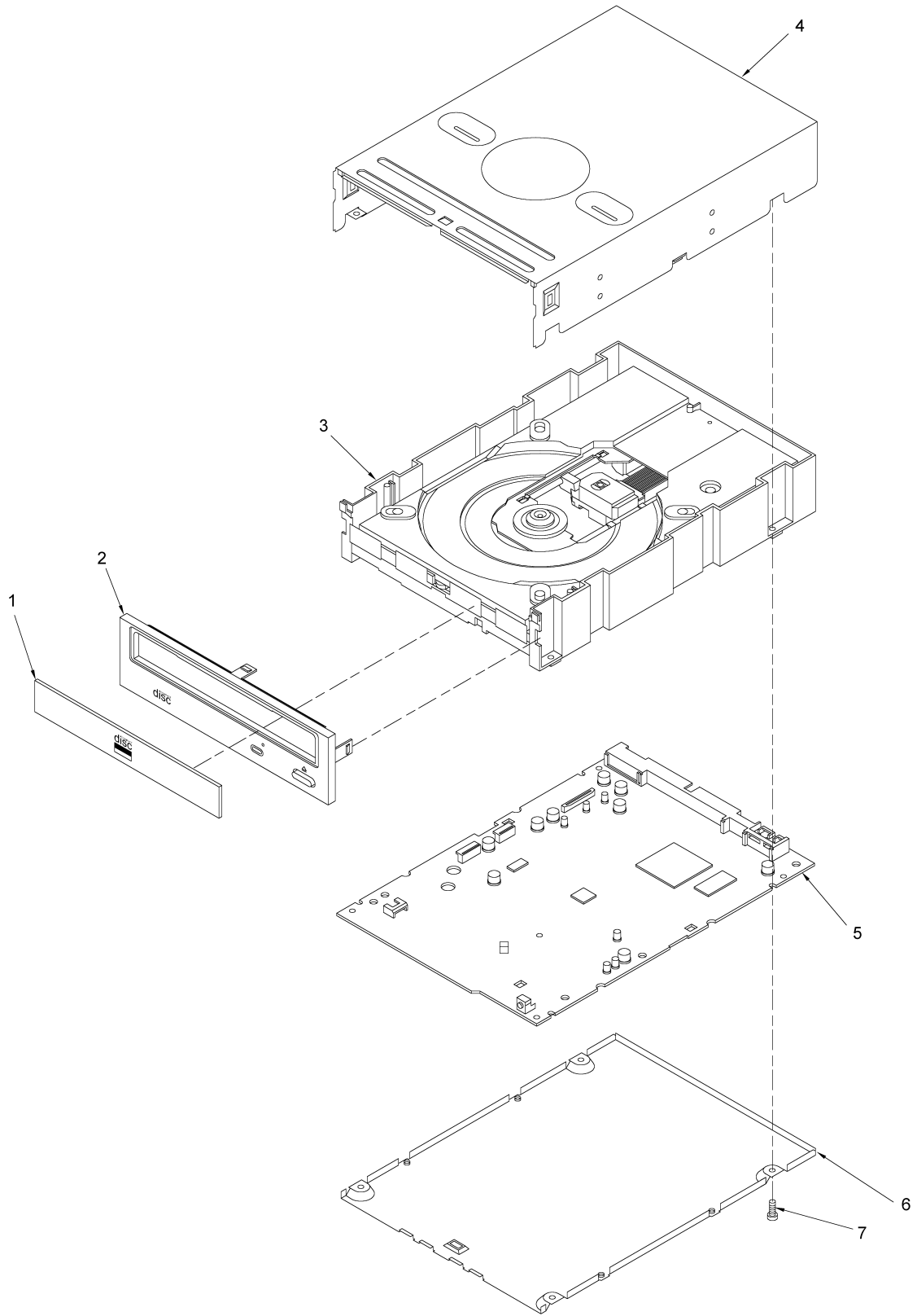
Figure 1. CD-ROM Drive Main Assembly
